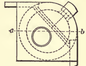
FIG. 5. STONE TOP INLET WITH CATCH-BASIN.
